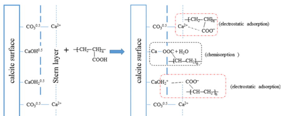
Fig. 10. Proposed models for the adsorption of PAA on calcite surface
