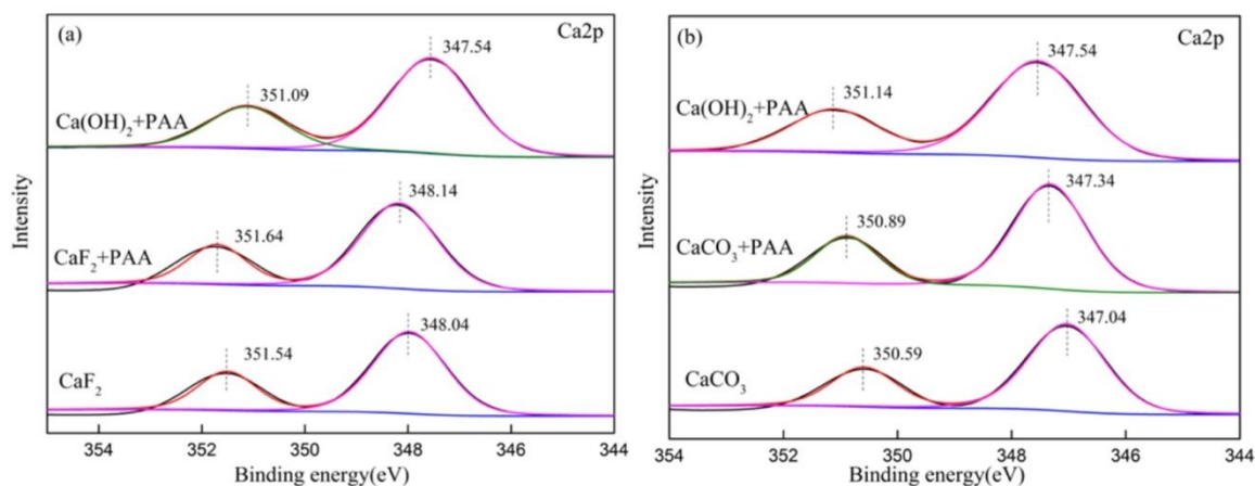
Fig. 7. Ca2p XPS spectra of fluorite (a) and calcite (b) samples
