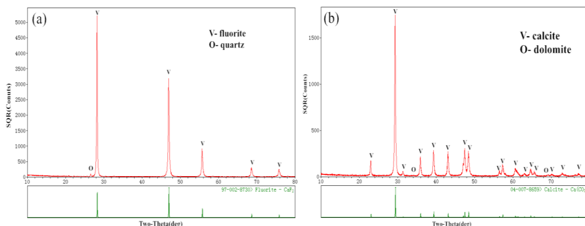
Fig. 1. XRD spectra of the fluorite (a) and calcite samples (b) used for the flotation tests
