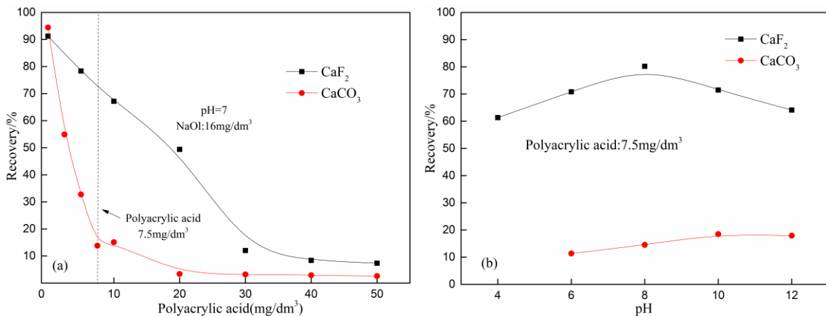
Fig. 3. Recovery of fluorite and calcite as a function of polyacrylic acid concentration (a) pH (b)
