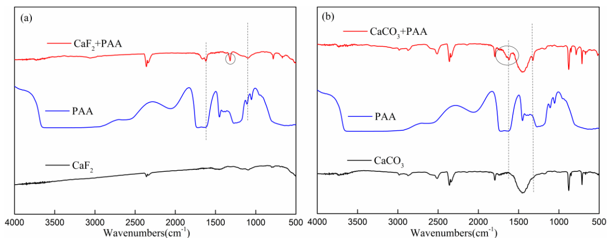
Fig. 5. FT-IR spectra of fluorite (a) and calcite (b) before and after interaction with polyacrylic acid
