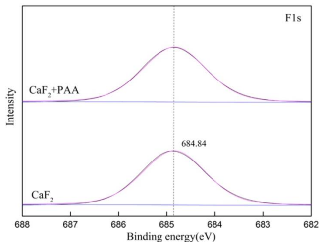
Fig. 8. F1s XPS spectra of fluorite
