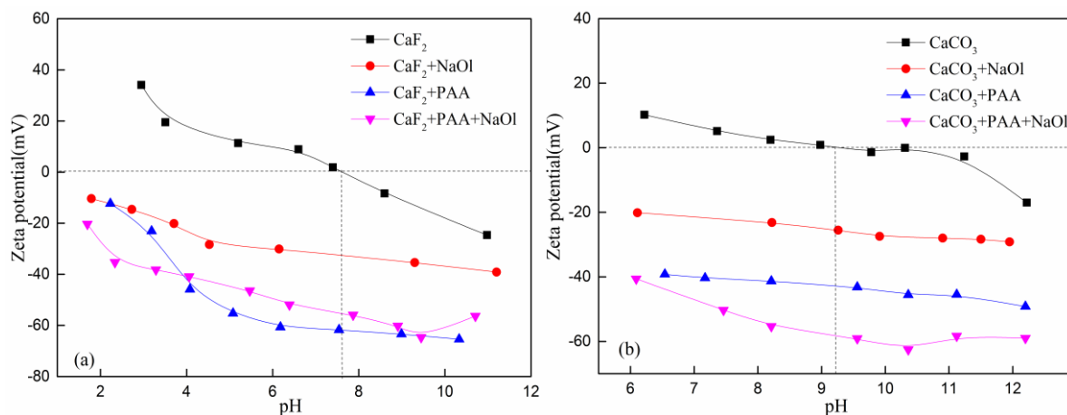
Fig. 4. Effect of the addition of different reagents on the zeta potentials of the minerals fluorite (a) calcite (b) (polyacrylic acid concentration=7.5 mg/dm 3 )
