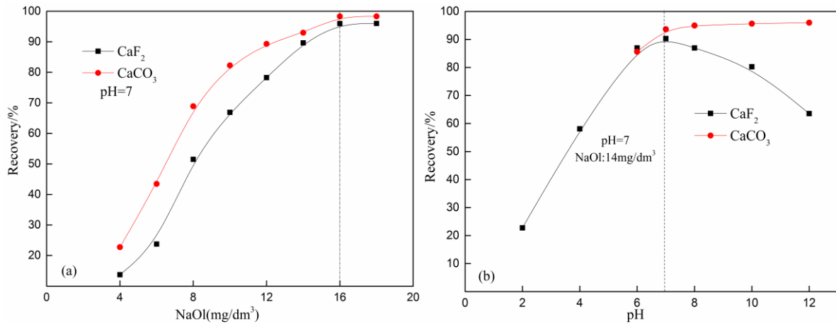
Fig. 2. Recovery of fluorite and calcite as a function of NaOl concentration (a) pH (b)
