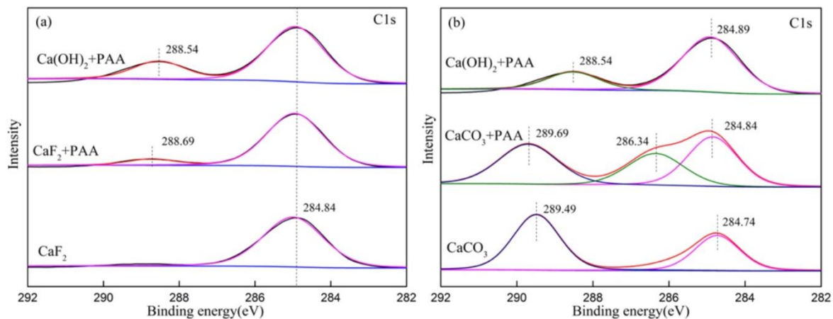
Fig. 6. C1s XPS spectra of fluorite (a) calcite (b)
