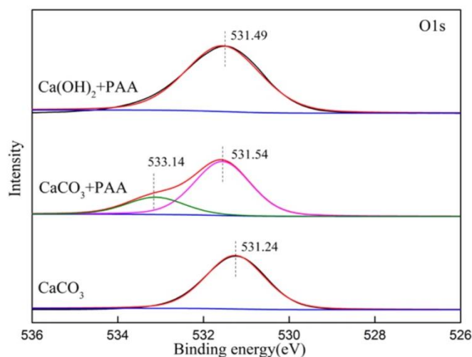
Fig. 9. O1s XPS spectra of calcite
