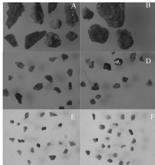
Fig. 3. Representative pictures of crushed chromite samples at different size ranges (A, C and E particles in 1+0.5; -0.5+0.212 and -0.212 mm size range with compressive breakage, B, D and F particles in 1+0.5; -0.5+0.212 and -0.212 mm size range with impact breakage)
