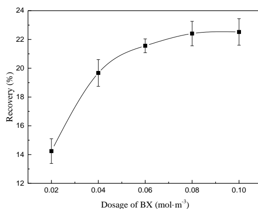
Fig. 4. Effect of BX on flotation recovery of cyanide chalcopyrite
