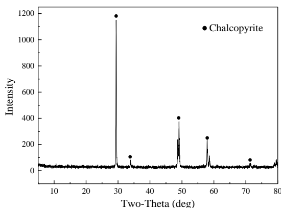
Fig. 1. XRD analysis of single chalcopyrite mineral
