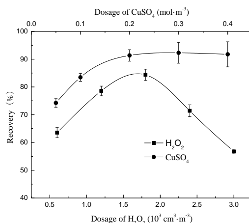
Fig. 5. Effect of \text{CuSO}_4 and \text{H}_2\text{O}_2 on the flotation recovery of cyanide chalcopyrite
