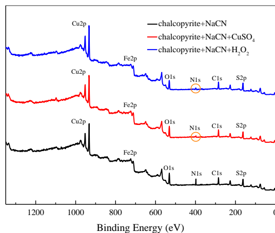
Fig. 7. XPS spectrum of chalcopyrite surface
