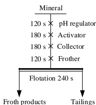
Fig. 2. The schematic of flotation test
