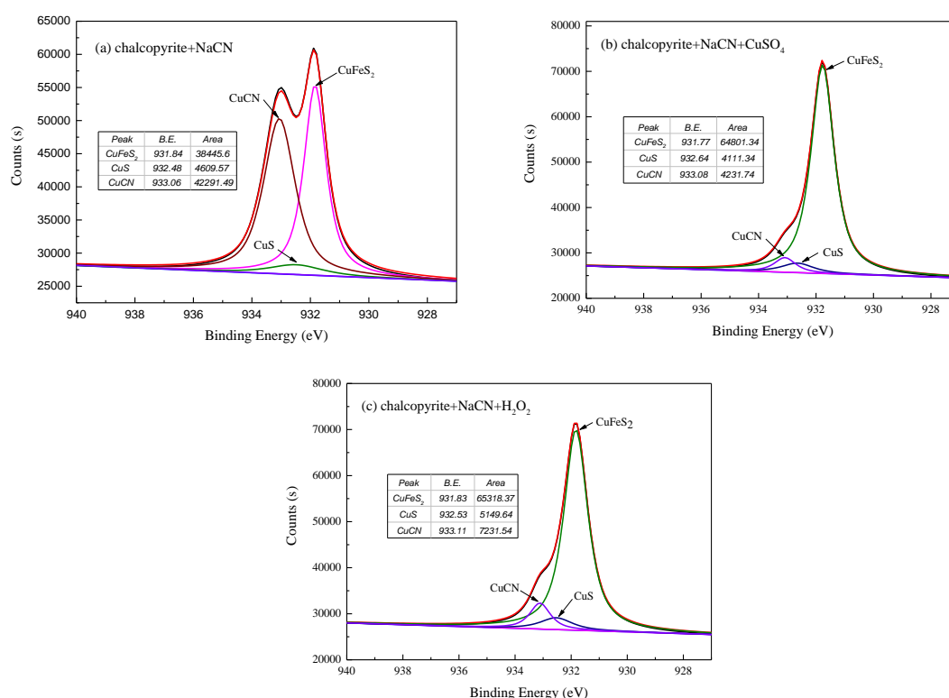
Fig. 8. XPS spectrum of Cu 2p on the surface of chalcopyrite before and after activation
