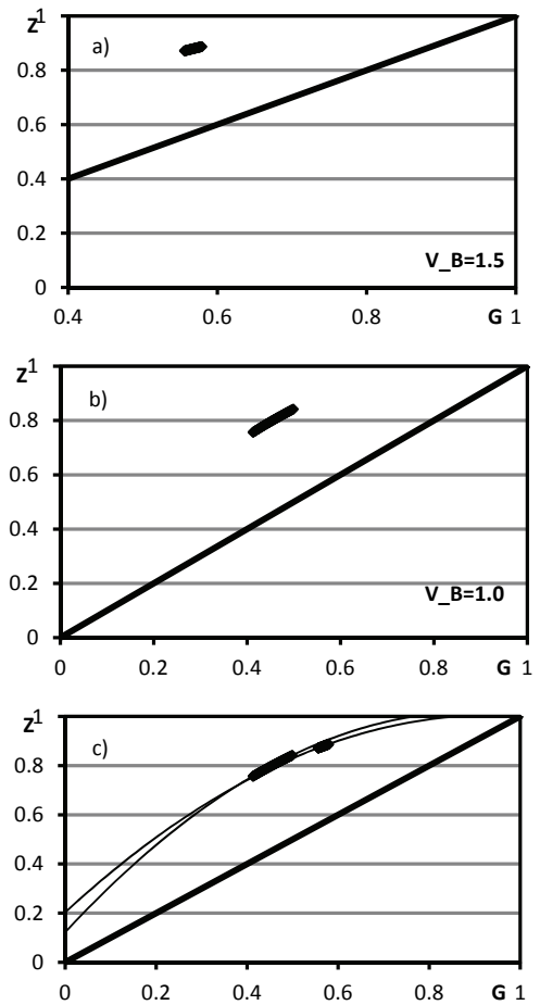
Fig. 18. Dependence of the Zenga and Gini indexes on skewness for a fixed value of variation, V_B = 1.5 and V_B = 1.0 for the Burr distribution. Source: authors' calculations
