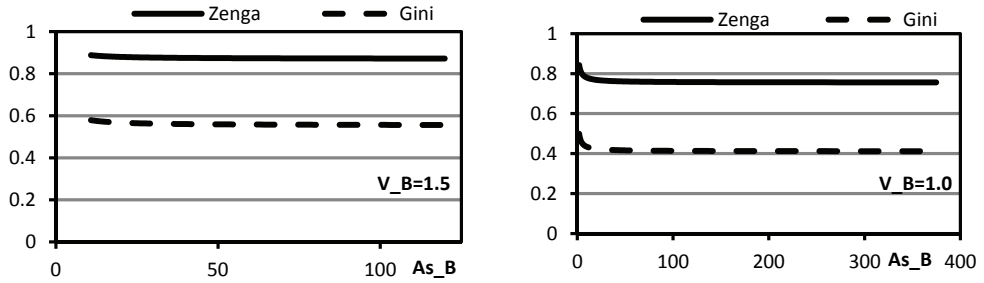
Fig. 18. Dependence of the Zenga and Gini indexes on skewness for a fixed value of variation, V_B = 1.5 and V_B = 1.0 for the Burr distribution. Source: authors' calculations
