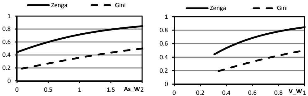
Fig. 11. Dependence of the Zenga and Gini indexes on skewness and variation for the Weibull distribution. Source: authors' calculations
