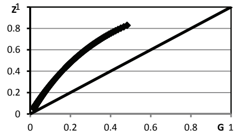
Fig. 5. Dependence of the Zenga index on the Gini index for the Gamma distribution. Source: authors' calculations
