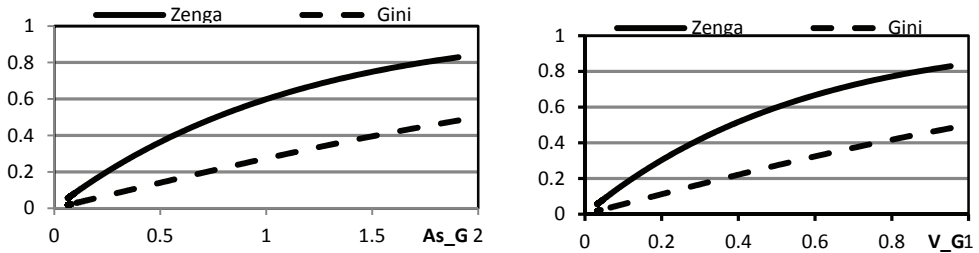
Fig. 4. Dependence of the Zenga and Gini indexes on skewness and variation for the Gamma distribution. Source: authors' calculations
