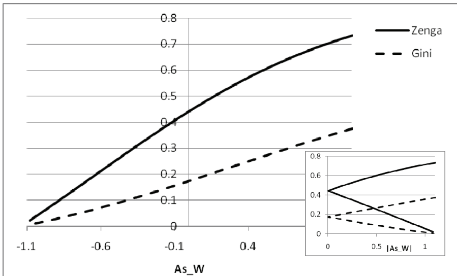
Fig. 13. Dependence of the Zenga and Gini indexes on the value of skewness and on the absolute value of skewness in the range of \alpha where it changes sign. Source: authors' calculations
