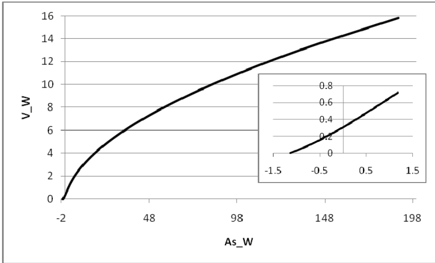
Fig. 10. The dependence of variation on the skewness for the Weibull distribution. Source: authors' calculations
