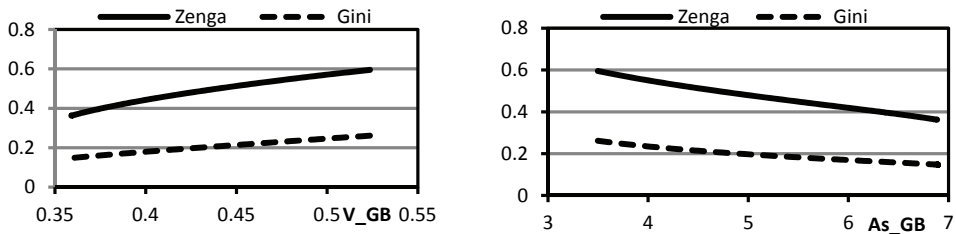
Fig. 21. Dependences of the Zenga and Gini indexes on variation (left) and skewness (right) for the generalized Burr distribution and a = 20, b = 3000, q = 0.2 with p ranging from 0.1 to 100.
