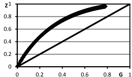
Fig. 2. Dependence of the Zenga index on the Gini index for the lognormal distribution Source: authors' calculations
