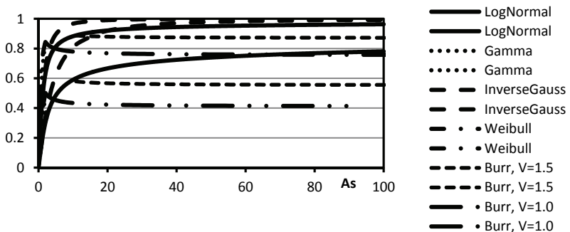
Fig. 23. Dependences of the Zenga and Gini indexes on skewness for various distributions. Source: authors' calculations
