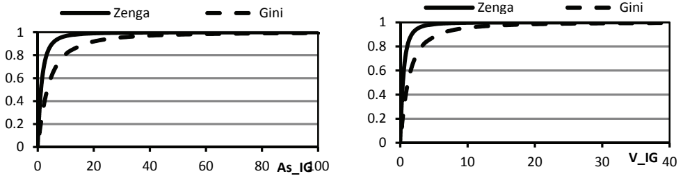
Fig. 7. Dependence of the Zenga and Gini indexes on skewness and variation for the inverse Gaussian distribution. Source: authors' calculations
