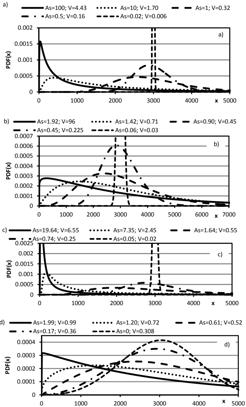
Fig. 20. Shape of the probability density function of the a) log-normal, b) Gamma, c) inverse Gaussian, d) Weibull distribution for a few values of skewness and variation. Source: authors' calculations
