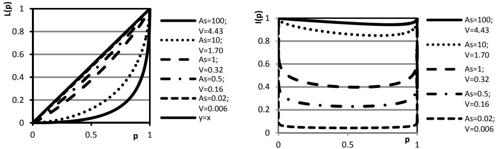
Fig. 3. The Lorenz and I(p) curves for the log-normal distribution for a few chosen values of skewness and variation. Source: authors' calculations
