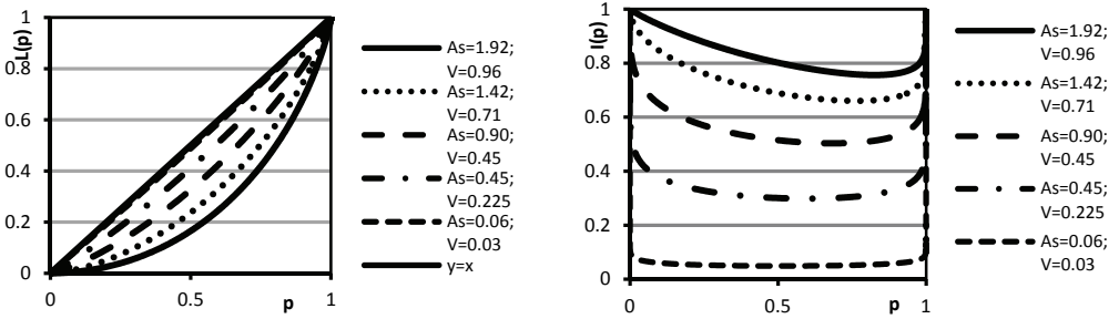
Fig. 6. The Lorenz and I(p) curves for the Gamma distribution for a few chosen values of skewness and variation. Source: authors' calculations
