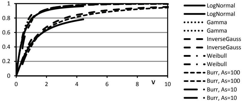
Fig. 22. Dependences of the Zenga and Gini indexes on variation for various distributions. Source: authors' calculations
