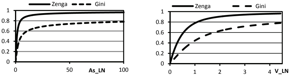
Fig. 1. Dependence of the Zenga and Gini indexes on skewness and variation for the log-normal distribution. Source: authors' calculations
