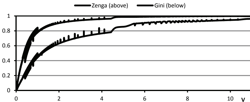
Fig. 24. Dependences of the Zenga and Gini indexes on variation for all the distributions considered.
