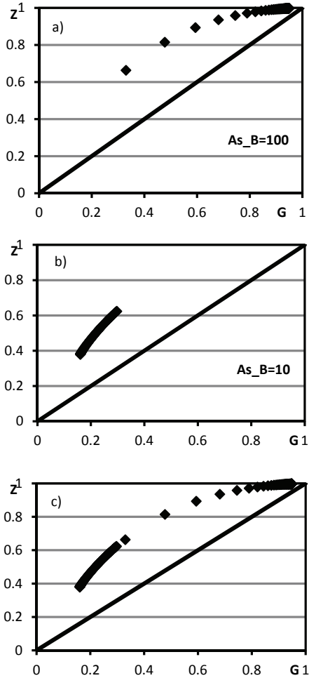
Fig. 17. Dependences of the Zenga index on the Gini index for the Burr distribution with fixed value of skewness, A_{S_B} = 100 , A_{S_B} = 10 , (a, b), and for both A_{S_B} = 100 , and A_{S_B} = 10 , (c). Source: authors' calculations
