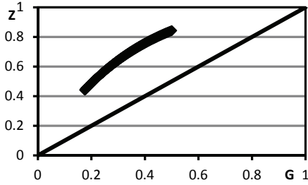
Fig. 12. Dependence of the Zenga index on the Gini index for the Weibull distribution. Source: authors' calculations
