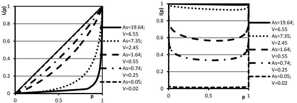
Fig. 9. The Lorenz and I(p) curves for the inverse Gaussian distribution for a few chosen values of skewness and variation. Source: authors' calculations
