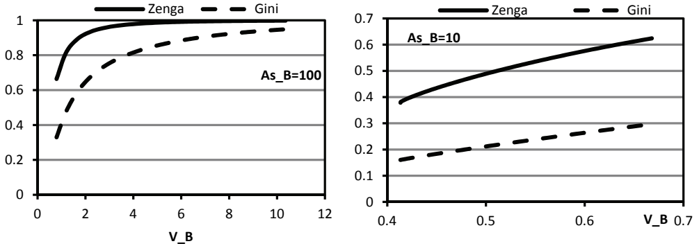
Fig. 16. Dependence of the Zenga and Gini indexes on variation for a fixed value of skewness, As_B = 100 and As_B = 10 for the Burr distribution. Source: authors' calculations
