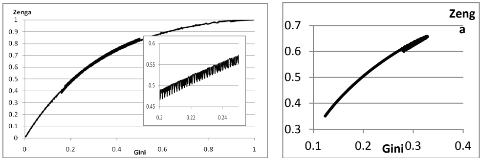
Fig. 26. Relation between the Zenga index and Gini index for a) unimodal distributions and b) bimodal distribution. Source: authors' calculations
