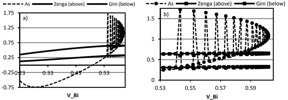
Fig. 25. The dependences of skewness, the Zenga index and Gini index with variation for a bimodal distribution. Source: authors' calculations
