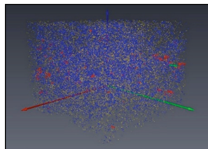
Fig. 7. Microtomographic image of Devonian sandstone pore space (subsample B); Avizo application, OGI-NRI in Cracow
