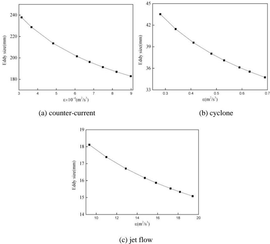
Fig. 17. Relationship between eddy size and \varepsilon
