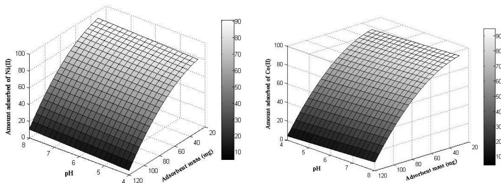
Fig. 2. Correlation between pH and adsorbent mass with adsorbed amount of metal ions
