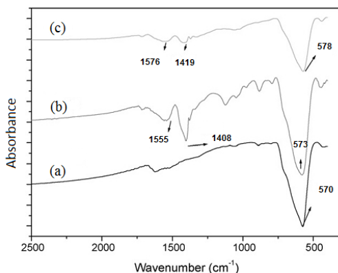
Fig. 4. FTIR spectra of (a) pure \text{Fe}_3\text{O}_4 , (b) \text{Fe}_3\text{O}_4 -chitosan and (c) \text{Fe}_3\text{O}_4 -carboxymethyl chitosan nano-adsorbents
