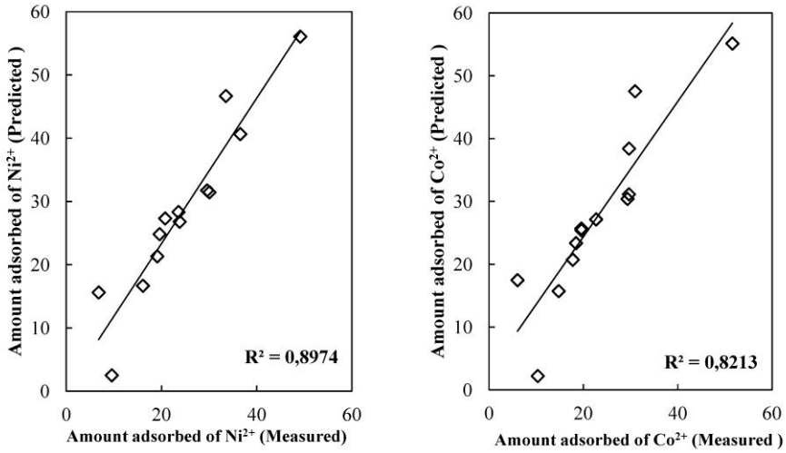
Fig. 6. Measured vs. predicted values of adsorbed amount of metal ions in the testing stage using the MNLR model
