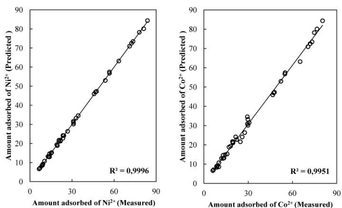
Fig. 8. Correlation between observed and predicted values in the training stage using the ANN model for nickel (left) and cobalt (right) ions
