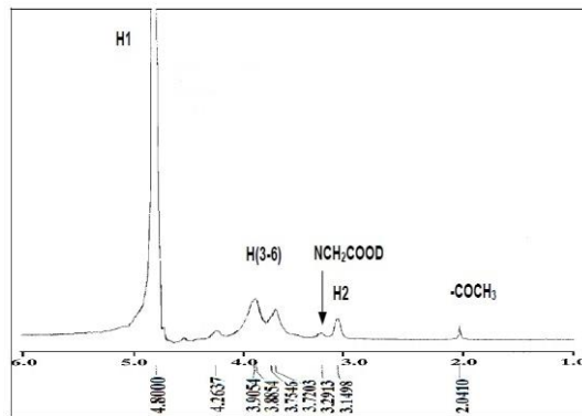
Fig. 5. H-NMR spectrum of carboxymethyl chitosan
