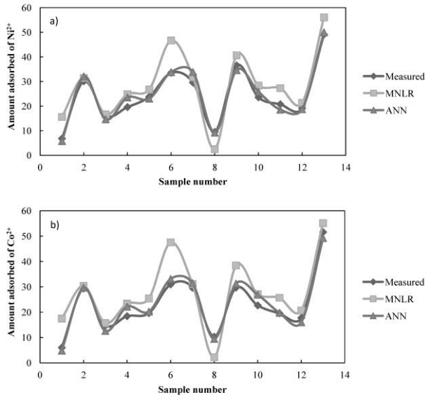
Fig. 10. Comparison of predicted and measured values for MNL and ANN models in testing stage, (above figure) adsorbed amount of Ni 2+ (a) Co 2+ (b) ions
