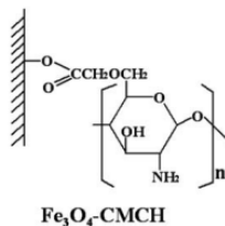
Fig. 1. Carboxymethyl chitosan-bounded Fe 3 O 4 nanoparticles (Chang et al., 2006)
