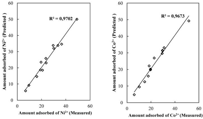
Fig. 9. Correlation between observed and predicted values in the testing stage using ANN model for nickel (left) and cobalt (right) ions
