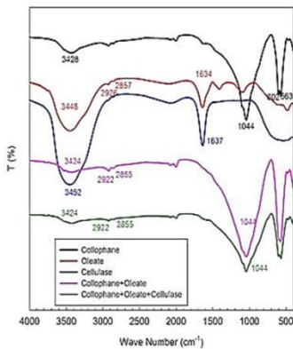
Fig. 5. FTIR spectra of collophane, oleate, cellulase and treated collophane
