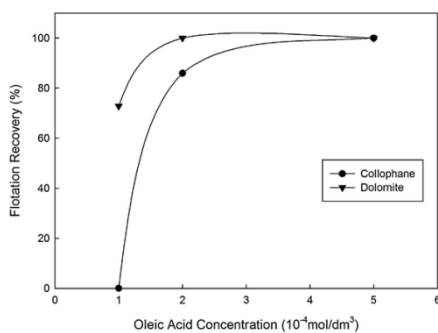
Fig. 1. Effect of oleate concentration on floatability of collophane and dolomite single minerals
