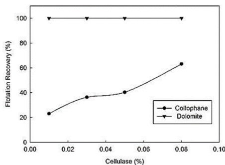
Fig. 2. Effect of cellulase concentration on floatability of collophane and dolomite single minerals using 2 \cdot 10^{-4} mol/dm 3 oleic acid
