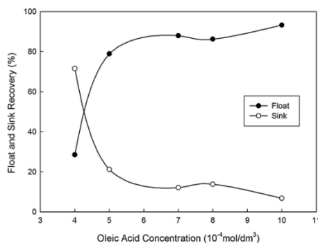
Fig. 8. Effect of oleic acid concentration on the flotation of Abu-Tartur phosphate ore sample
