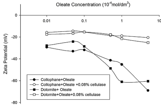
Fig. 4. Effect of different concentrations of oleate and oleate/0.08% cellulase on zeta potential of collophane and dolomite at pH 6
