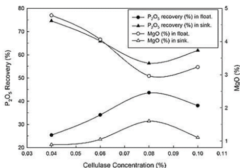
Fig. 9. Effect of cellulase concentration on the flotation of Abu Tartur phosphate ore
