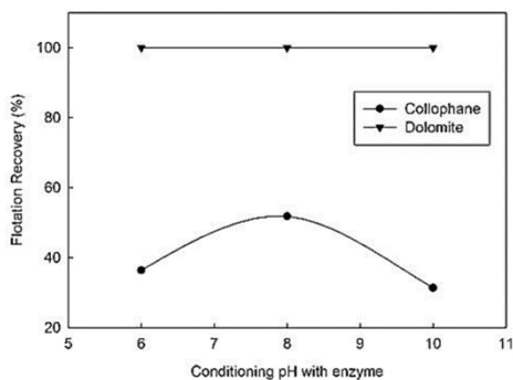
Fig. 3. Effect of conditioning pH, with enzyme, on floatability of collophane and dolomite single minerals in presence of cellulase using 2 \cdot 10^{-4} mol/dm 3 oleic acid
