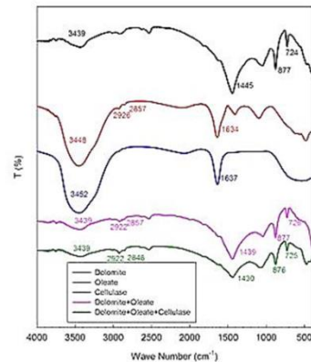
Fig. 6. FTIR spectra of dolomite, oleate, cellulase and treated dolomite
