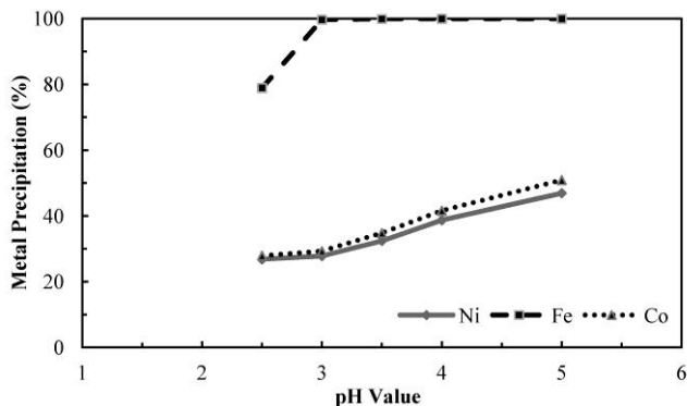
Fig. 1. Effect of pH on iron precipitation (60 min, without heating)
