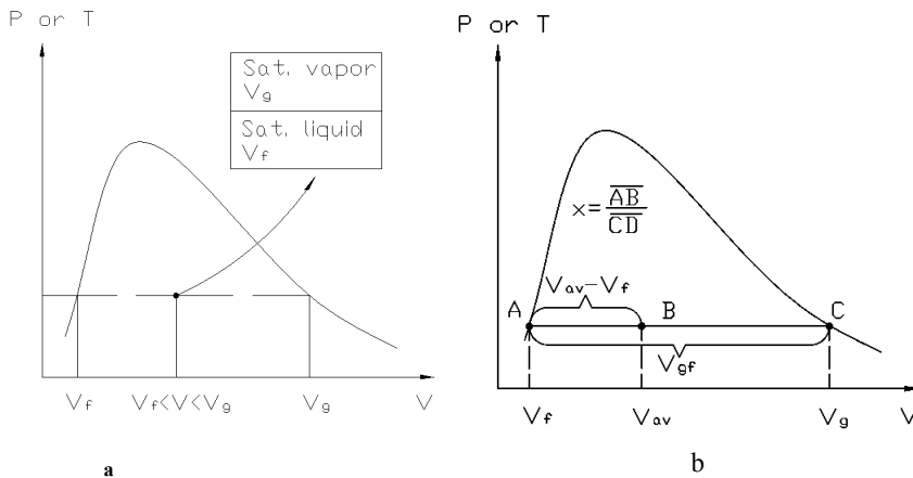
Fig.30a. The value of a saturated liquid –vapor mixture lies between the v_f and v_g values at the specified T or p; b) Quality is related to the horizontal distance on p-v and T-v diagrams.
