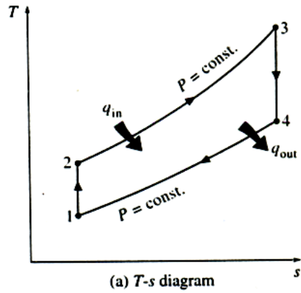
Figure 48A P-v diagrams for the ideal Figure 48B T-s diagrams for the ideal Brayton cycle
