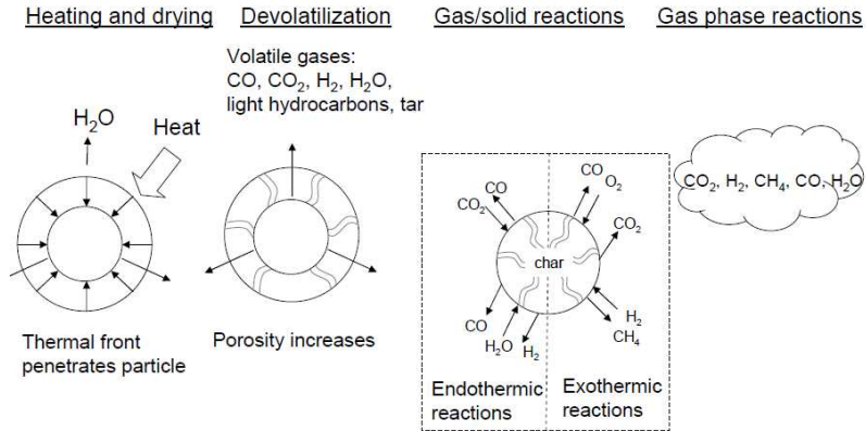
Fig.27. Mechanism of gasification process.
