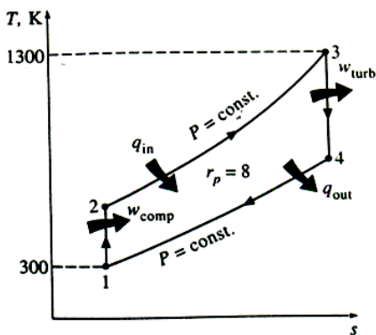
Figure 54 T-s diagram for the Brayton cycle discussed in example 6-1
