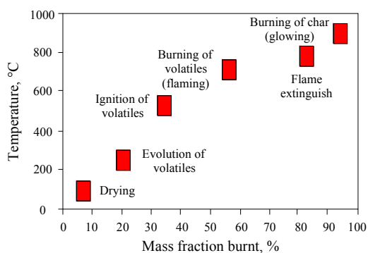
Fig. 25. Schematic description of the combustion process of a lump of straw or wood chip, according to Hellwig [42]
