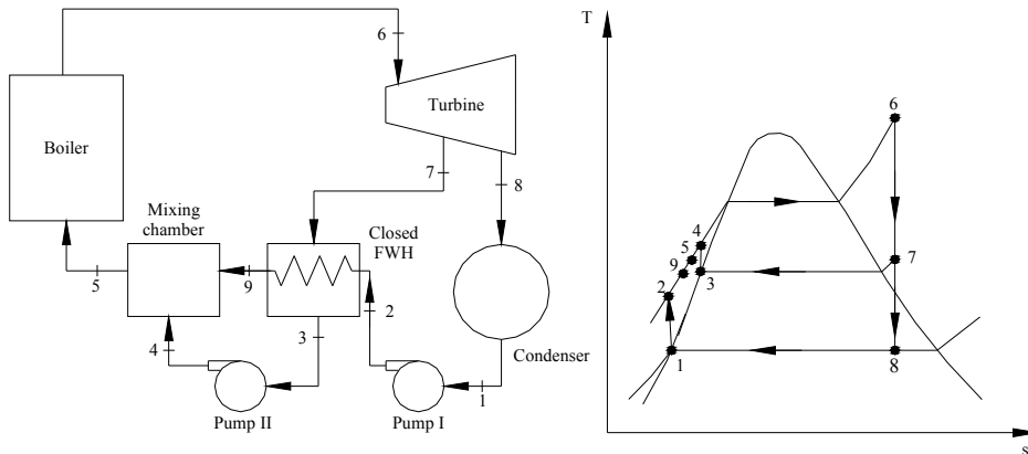
Figure 39. The ideal regenerative Rankine cycle a closed feedwater heater
