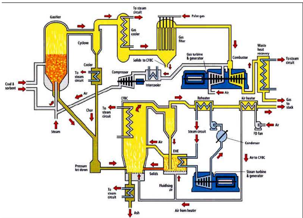
Figure 64. A schematic of the ABGC - Hybrid cycles
