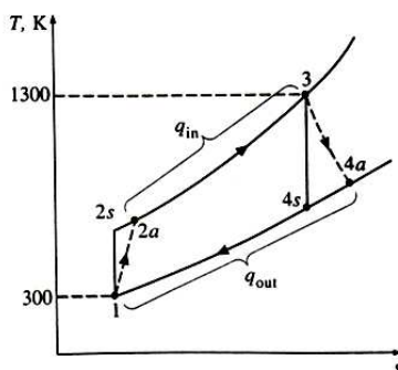
Figure 55 T-s diagram of the gas-turbine cycle discussed in Example 6-2
