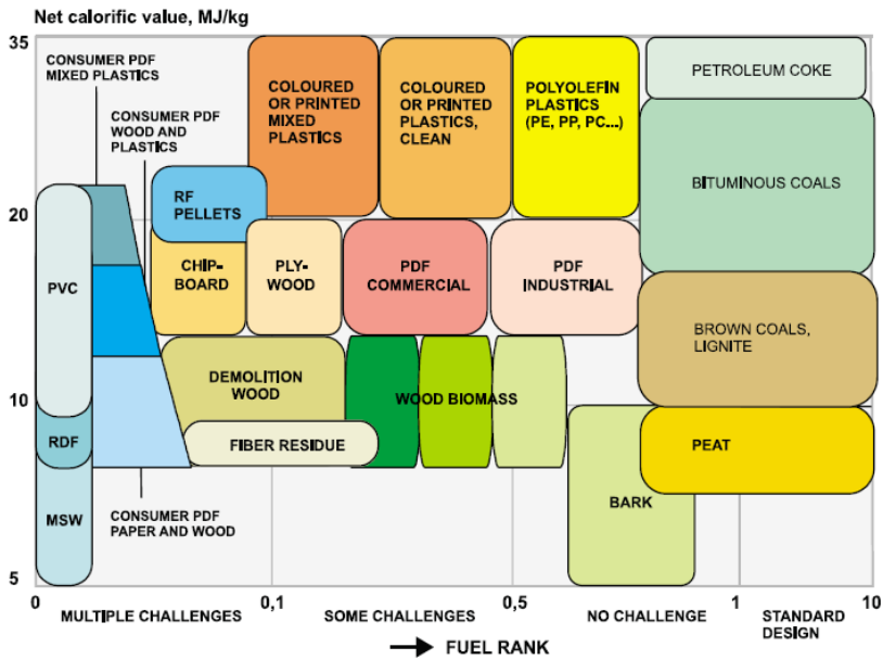
Fig. 7. Influence of fuel characterization to boiler design [7]
