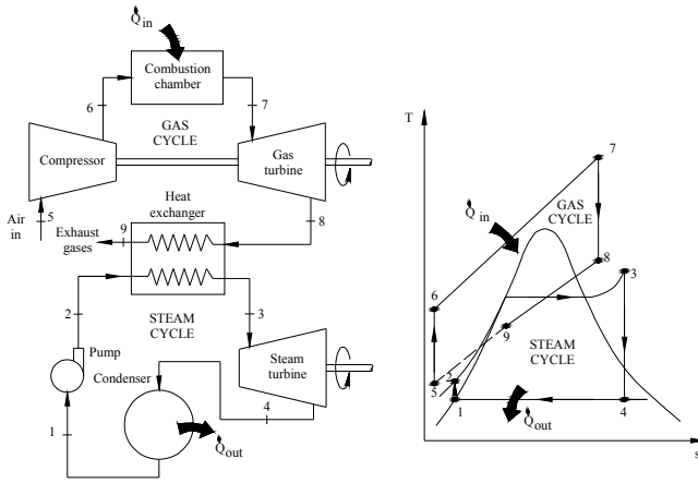
Figure 56 Combined gas-steam power plant
