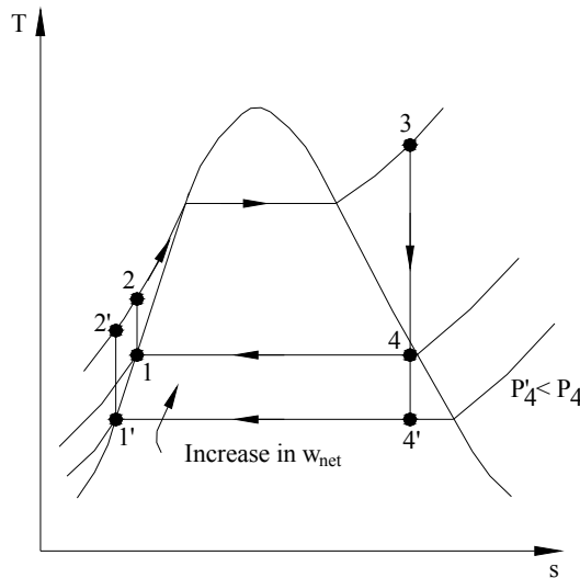
Fig. 31. The effect of lowering the condenser pressure on the ideal Rankine cycle
