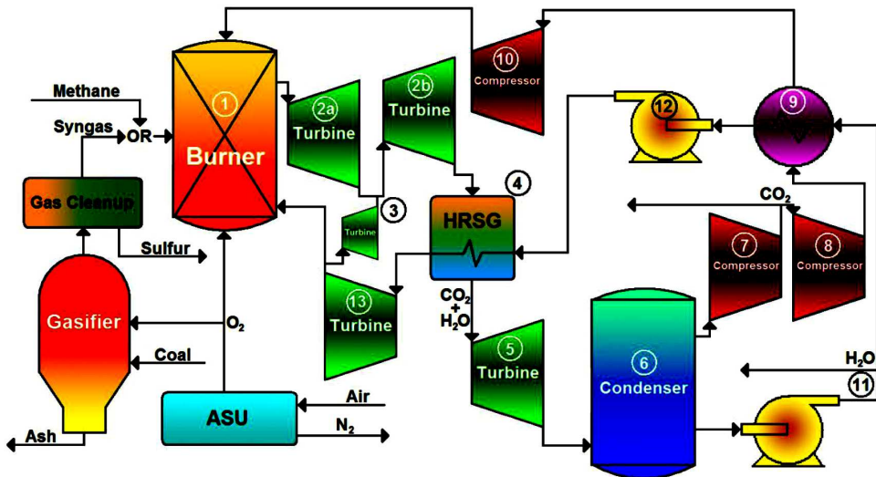
Figure 60 b . The IGCC plant scheme with oxygen gasification –Graz cycle
