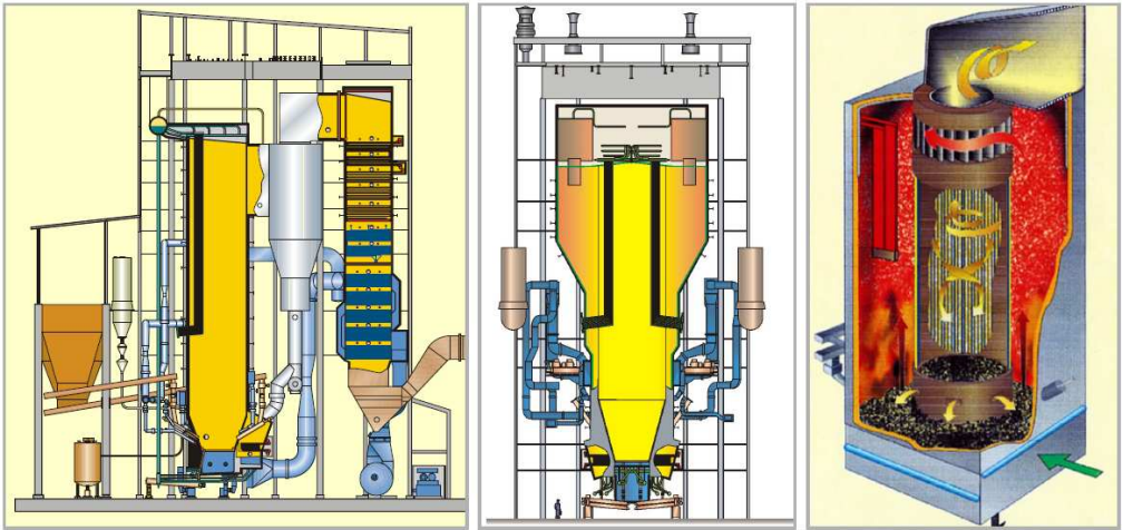
Figure 68. The technical schemes of CFB- boilers; with cyclone, compact boiler and bubbling fluidized bed.
