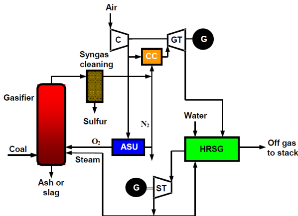
Figure 60a . The basic IGCC plant.
