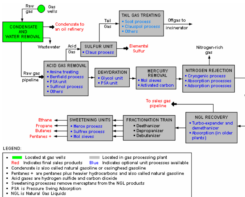
Fig. 15. Schematic flow diagram of a typical natural gas processing plant.
