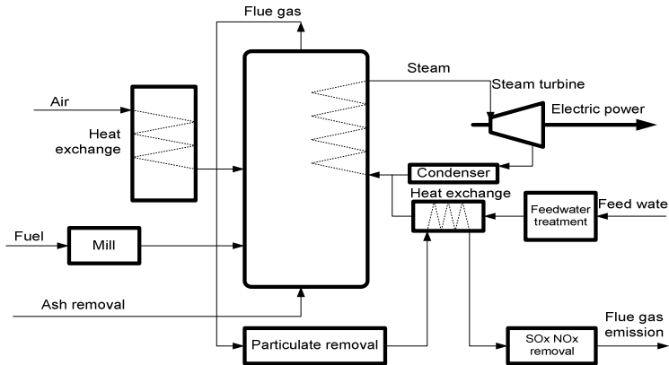
Fig.3. Scheme of Power Generation Plant fired with fossil fuel ( Thermal Power Plant).
