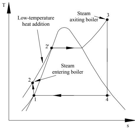
Figure 38. The first part of the heat-addition process in the boiler takes place at relatively low temperatures
