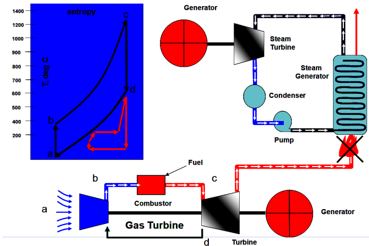
Fig. 57. Scheme of combined power plant with diagram of thermodynamic cycle
