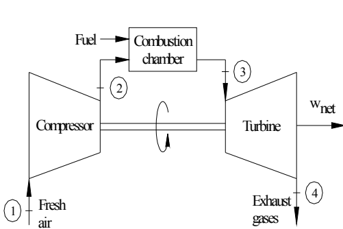
Figure 46 An open-cycle gas-turbine engine
