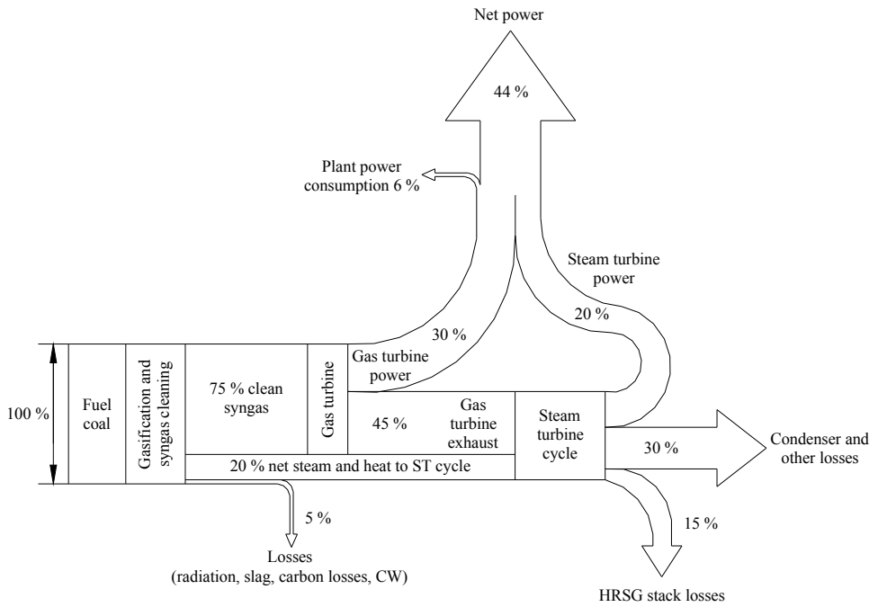
Figure 61. Energy flow diagram for IGCC.
