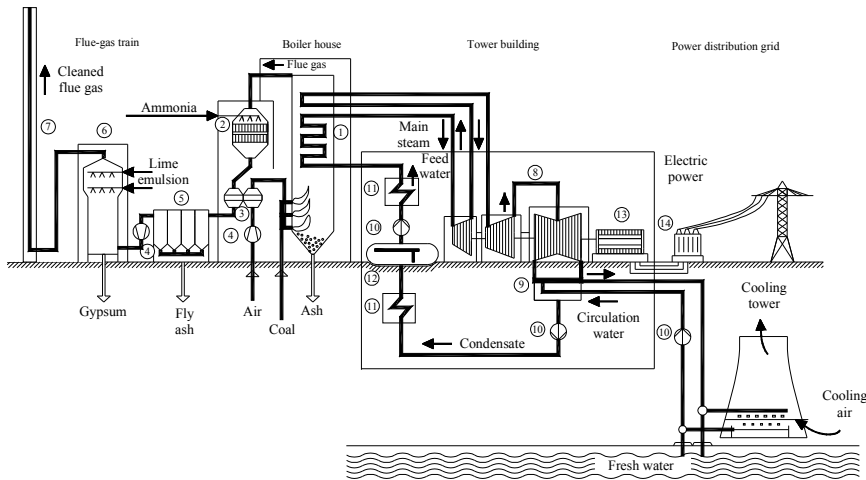
Figure 41. Advanced pulverized coal-fired power plant [52]
