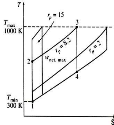
Figure 50. For fixed values of T_{\min} and T_{\max} , the net work of the Brayton cycle first increases with the pressure ratio, then reaches a maximum at r_p = (T_{\max}/T_{\min})^{-1/k/[2(k-1)]} and finally decreases
