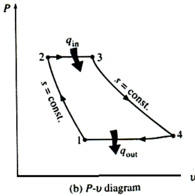
Figure 48A P-v diagrams for the ideal Figure 48B T-s diagrams for the ideal Brayton cycle
