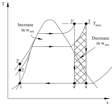
Fig. 33. The effect of increasing the boiler pressure on the ideal Rankine cycle
