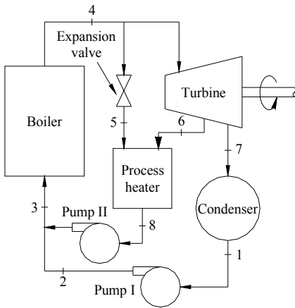
Figure 45. A cogeneration plant with adjustable loads
