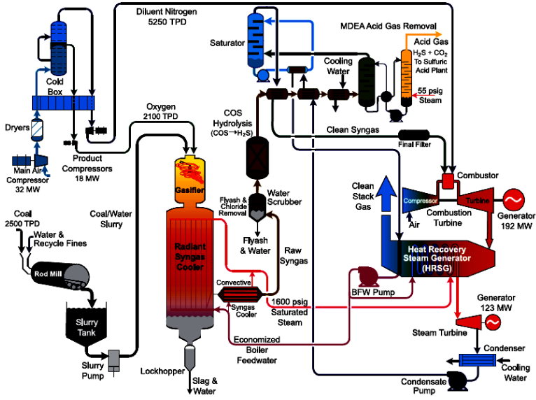
Figure 60c . The IGCC plant with gasification of slurry coal with oxygen and using nitrogen from separation of air in gas turbine with cleaned syngas from gasification.
