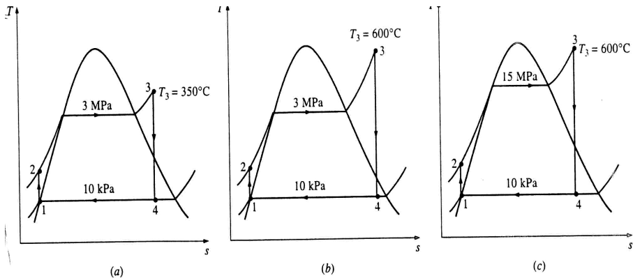
Fig.35.T-s diagrams of three cycles.
