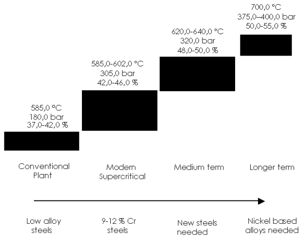
Figure 65. Development targets steam temperature and pressure.
