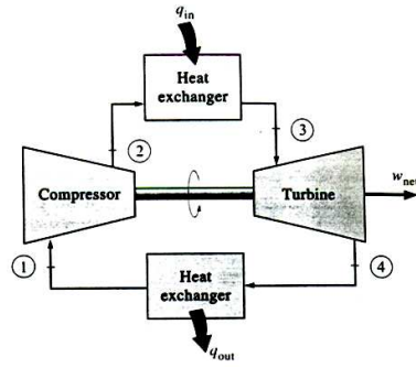
Figure 47 A closed-cycle gas-turbine engine
