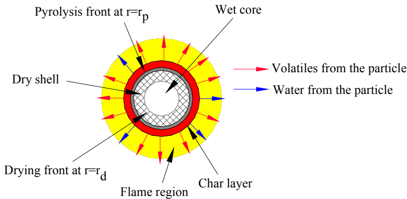
Fig. 26. Schematic diagram showing the combustion of a small biomass particle (i.e. with a 20 mm diameter) [46].
