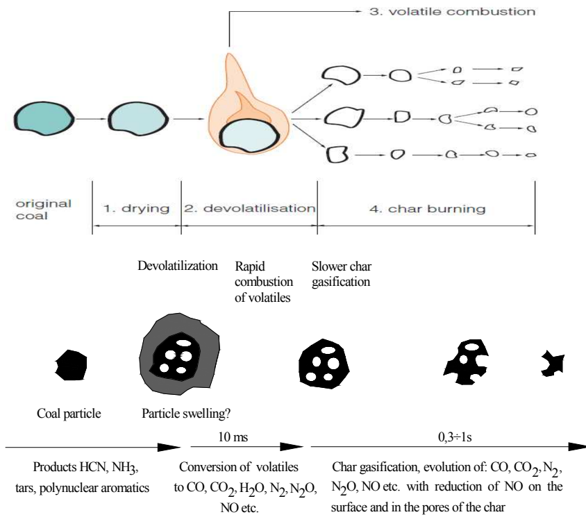
Fig. 12. Schematic representation of the processes occurring in the combustion of a single coal particle, according to Thomas [32]
