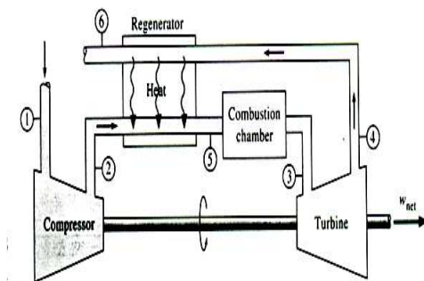
Figure 51 A gas-turbine engine with regenerator
