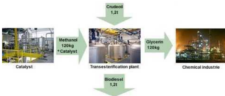
Fig. 20. Mass balance of biodiesel processing .
