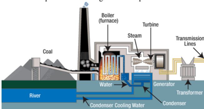
Fig. 4. Scheme of main units of thermal power plants fuelled coal..
