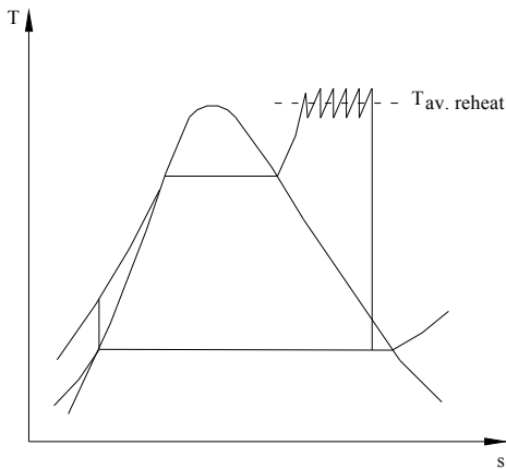
Figure 37. The average temperature at which heat is transferred during reheating increases as the number of reheat stages is increased
