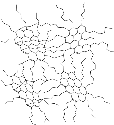
Fig. 9. Model of the polymeric structure of vitrinite, according to Kasatoczkin [9]
