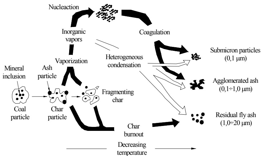
Fig. 14. Mechanisms of formation of ash particles, according to Helble et al. [34]
