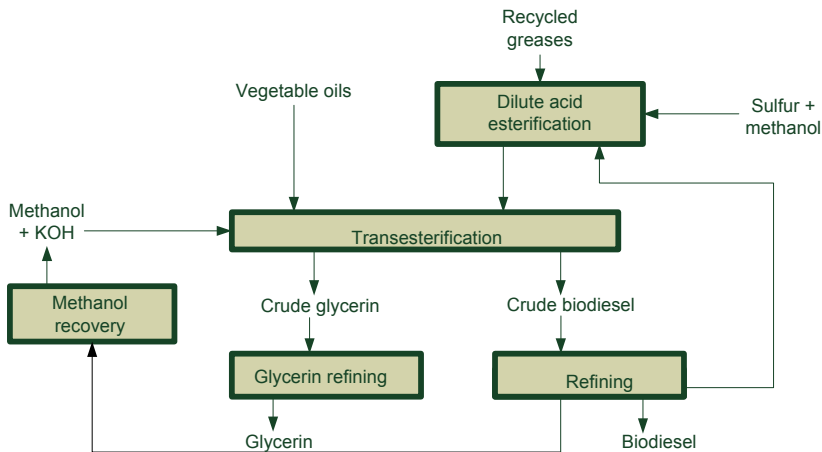
Fig. 19. Basic transesterification technology.
