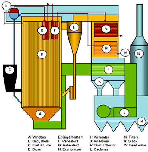
Figure 67. The base component of CFB boiler ( cyclone type ).
