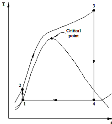
Fig. 34. A supercritical Rankine cycle.
