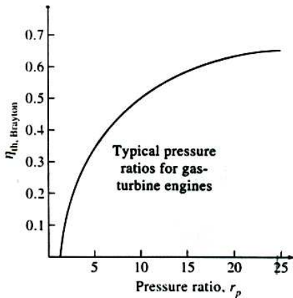
Figure 49. Thermal efficiency of the ideal Brayton cycle as a function of the pressure ratio
