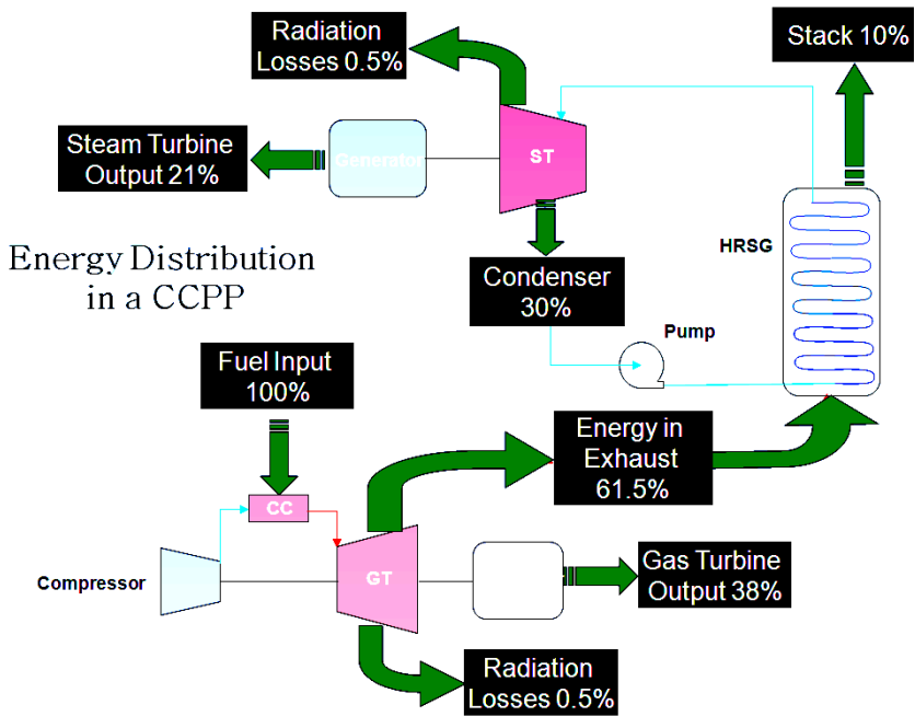
Figure 59. Balance energy for combined cycle
