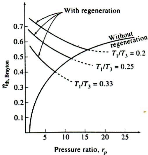
Figure 53 Thermal efficiency of the ideal Brayton cycle with and without regeneration
