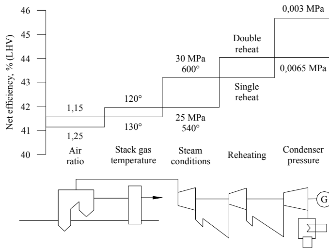
Figure 42 Effect of various measures for improving the efficiency (LHV) of pulverized coal-fired power generating plant [51].
