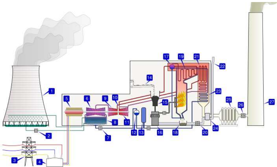
Fig. 5. Scheme of power unit – structure
