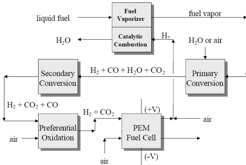
Fig. 18. Schematic of fuel processor/fuel cell power system [45].
