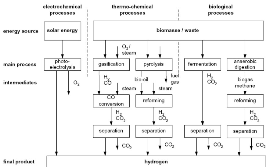
Fig. 16. Main processes for direct production of hydrogen from renewable energy sources [6]
