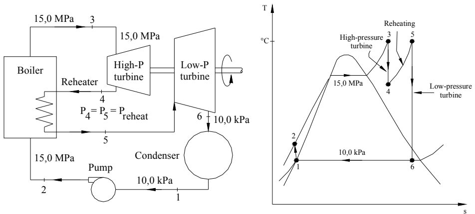
Figure 36. Schematic and T-s diagram for ideal reheat.
