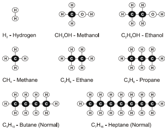
Fig.17. Chemical Structure of Common Fuels
