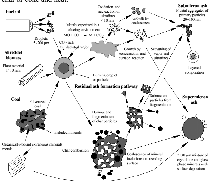
Fig. 13. Particle formation mechanisms, according to Huffman et al. [33]
