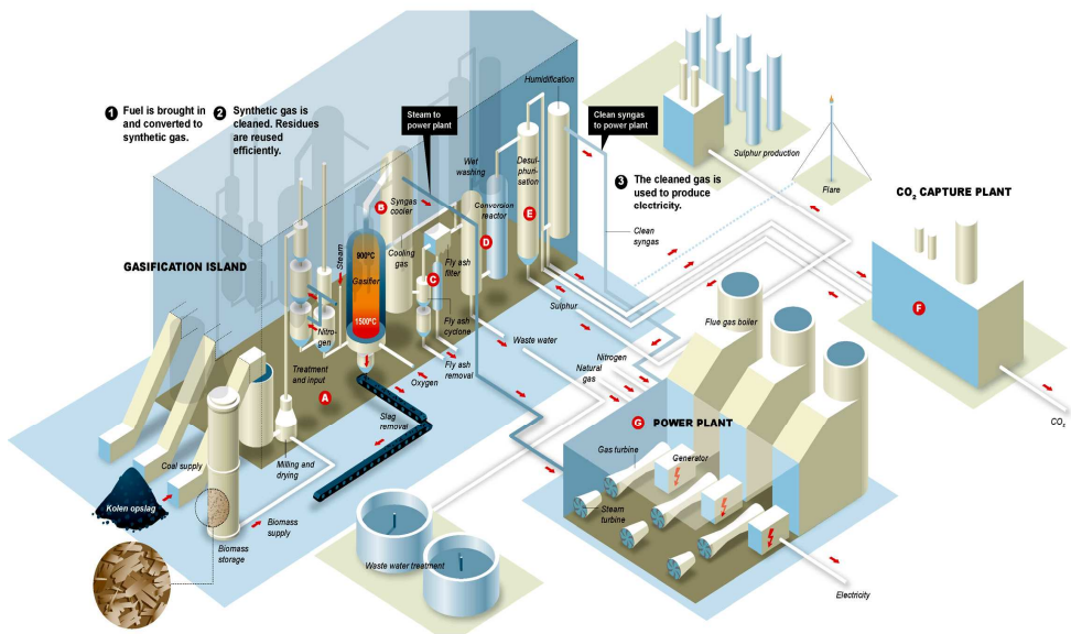
Fig.63. The scheme of IGCC process with co-gasification biomass and coal.
