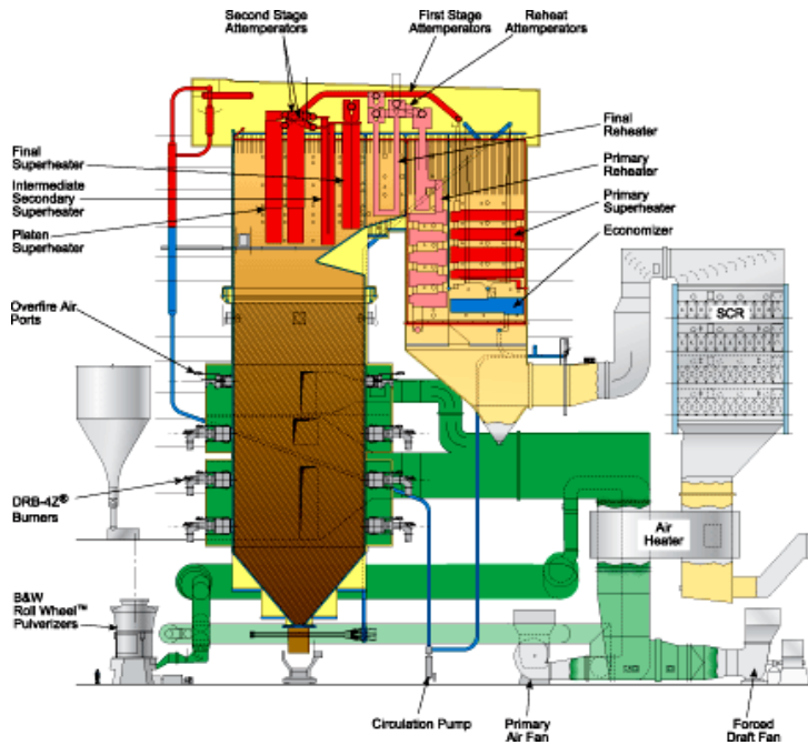
Fig.43. SC boiler with spiral tubes in furnace.
