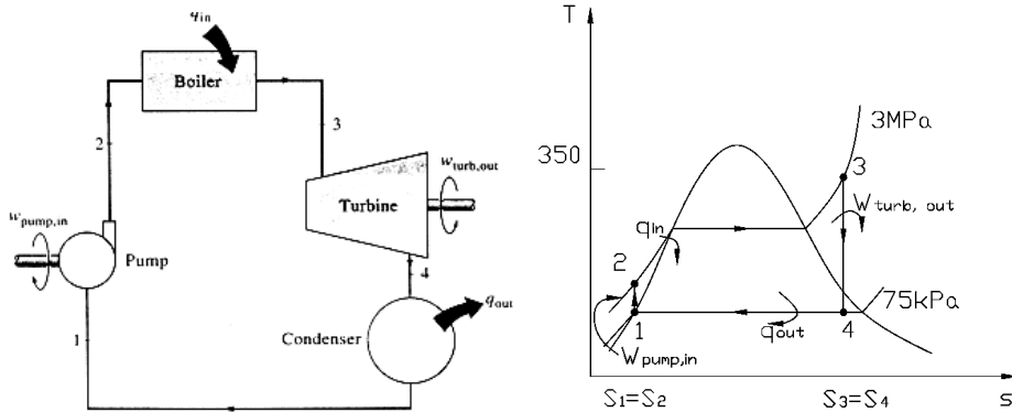
Fig. 29. The simple ideal Rankine cycle.
