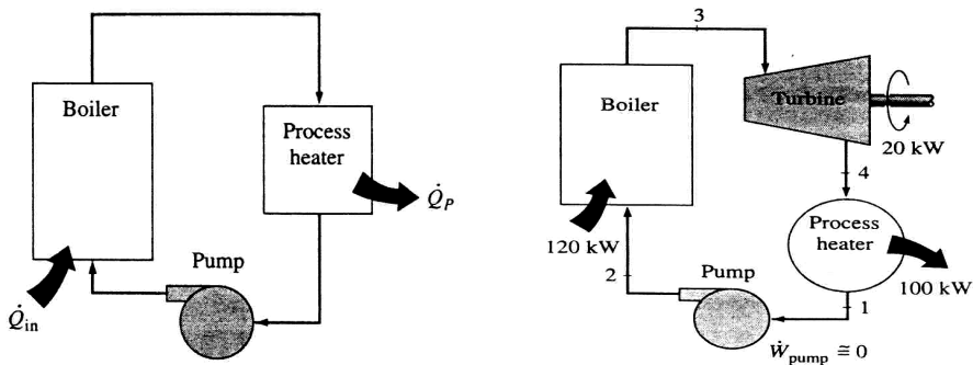
Figure 44a. A simple process-heating plant Figure 44b. An ideal cogeneration plant
