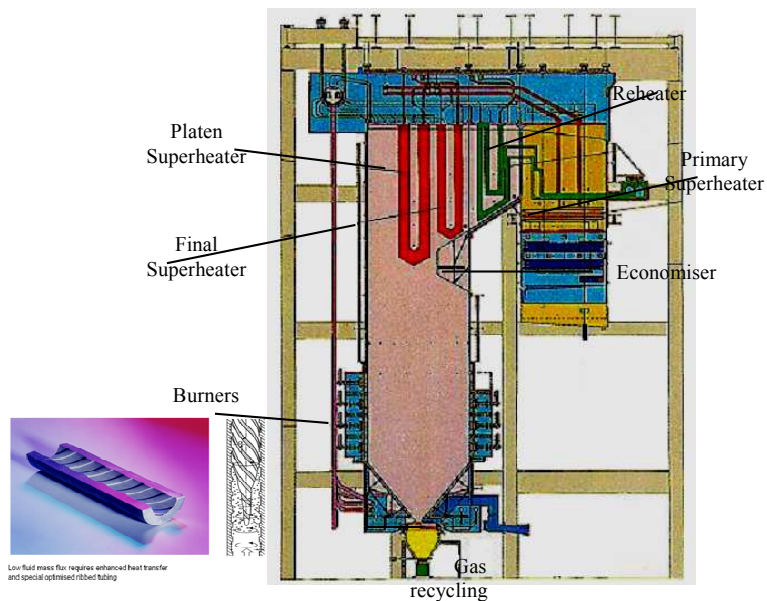
Figure 66. Supercritical boilers for advanced power production technology with optimized ribbed tubing for vertical tube furnace.
