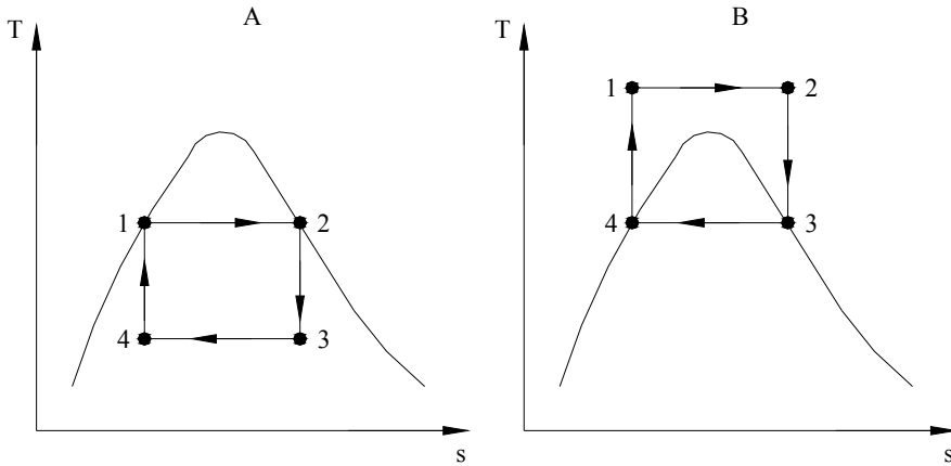
Fig. 28. A & B. T-s diagram of two Carnot vapor cycles
