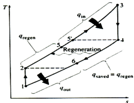
Figure 52 T-s diagram of a Brayton cycle with regeneration
