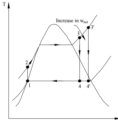
Fig. 32. The effect of superheating the steam to higher temperatures on the ideal Rankine cycle
