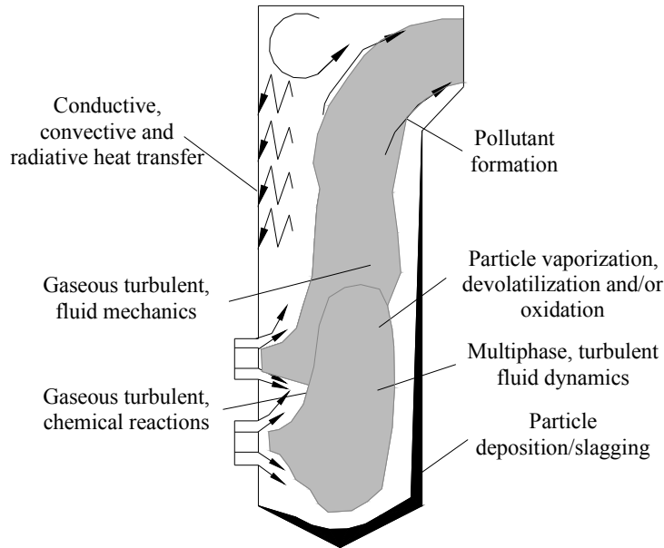
Fig. 11. Major physical and chemical mechanisms in a pulverized-coal combustion process, according to Eaton et al. [22]
