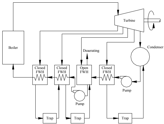
Figure 40. A steam power plant with one open and three closed feedwater heaters
