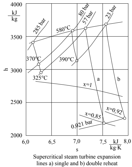
Figure 37a. Temperature entropy ( T, s ) diagram of SC cycle with double reheat. Figure 37b. Enthalpy entropy ( h, s ) representations of SC cycle with reheat [51]
