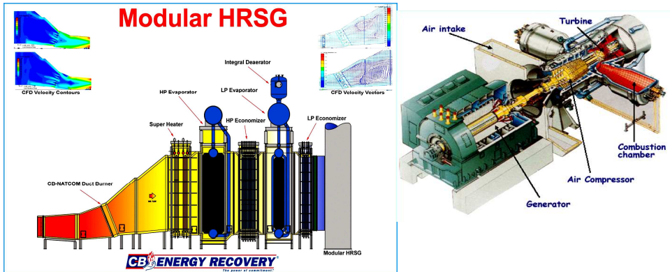
Figure 58. Scheme of heat generating steam generator and view of gas turbine .
