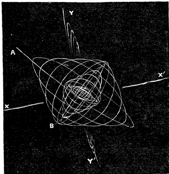
FIG. 14.—Specimen (obtained from nature) of the path of a stiff vibrating hazel shoot. Much friction. A, the starting-point. B, the end of the first cycle. xx' , the path of the twig set vibrating exactly in the plane of slow vibration. yy' , nearly in the plane of quick vibration.
