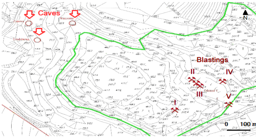
Fig. 12. Location of blasting in relation to delay nearest caves
