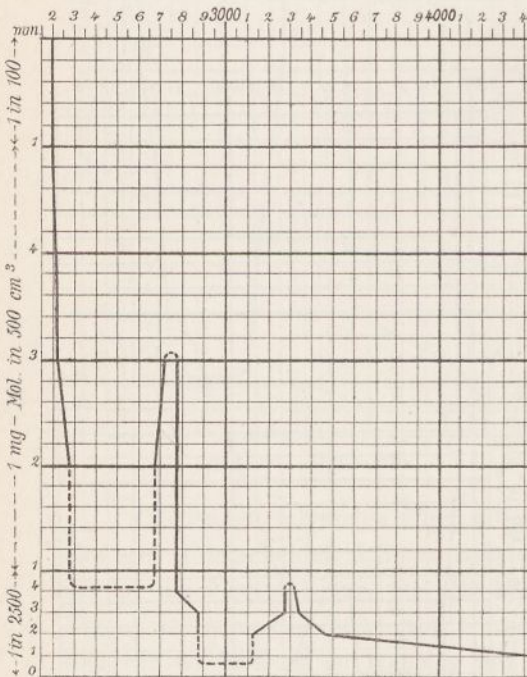
Fig. 66. Dehydrocorydalin nitrat.
