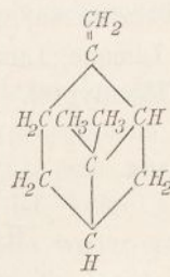
\Delta^{1\gamma} Camphen
