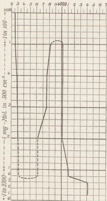
Fig. 58. Tetrahydroberberin.
