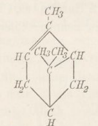
Pinen Camphen
