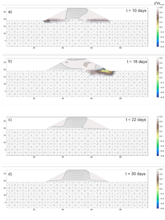
Figure 9: Maps of the normalised second-order work at different levels of the phreatic surface.
