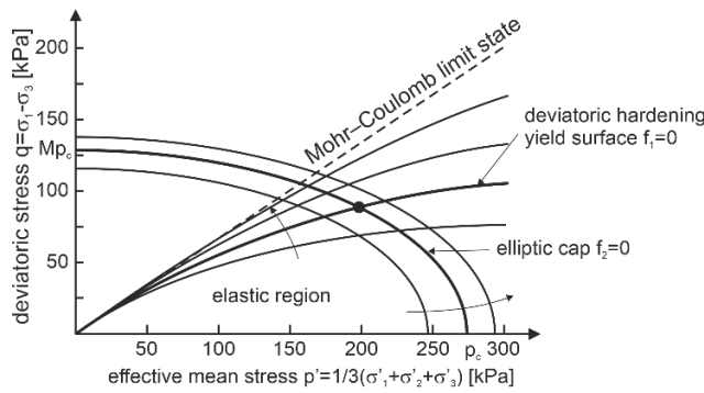
Figure 5: Yield surface for Hardening Soil model.
