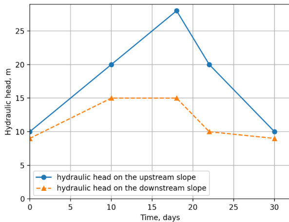
Figure 6: Variations of hydraulic boundary conditions over time.
