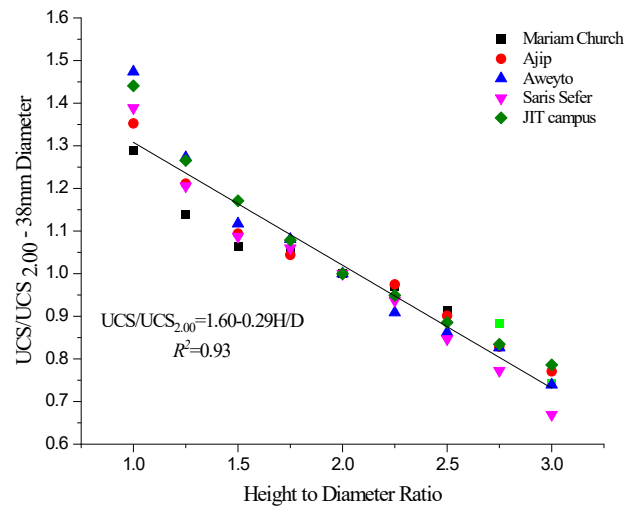
Figure 14: Plot of UCS/UCS_{2.00} versus height to diameter ratio for a specimen diameter of 38 mm.
