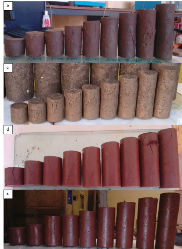
Figure 10: Failure pattern of 50 mm specimen diameter: (a) Ajip, (b) Aweytu, (c) JIT campus, (d) Saris Sefer, and (e) Mariam Church.
