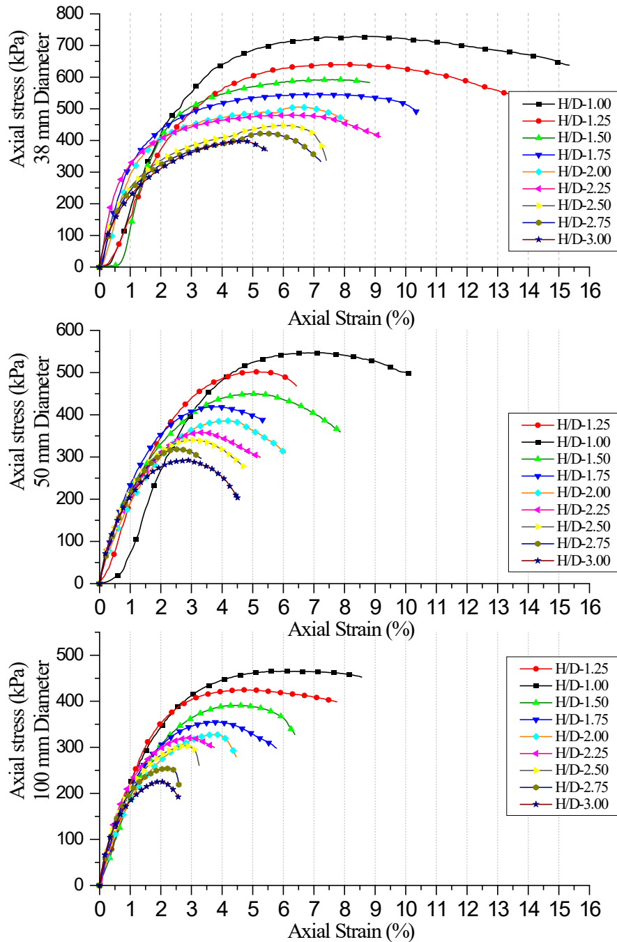
Figure 6: Stress–strain curves for 38 mm, 50 mm, and 100 mm specimen diameters of JIT campus test pit from top to bottom.
