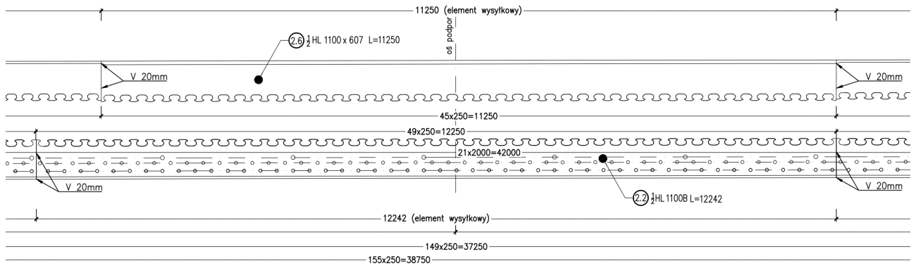
Figure 13: The geometry of the steel T-sections above the pillar [57].
