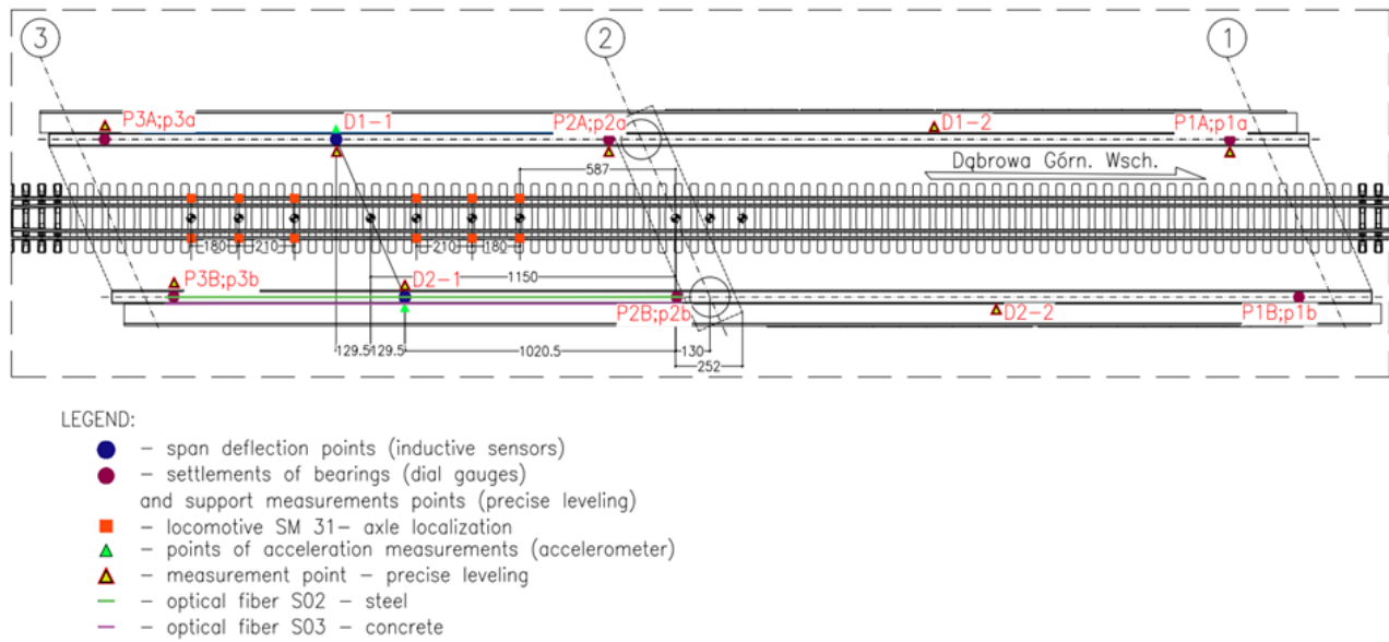
Figure 23: Load scheme and localization of measurements points.
