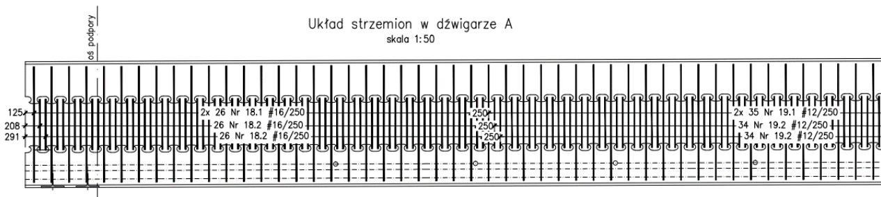
Figure 9: Shear reinforcement of hybrid girders [57].
