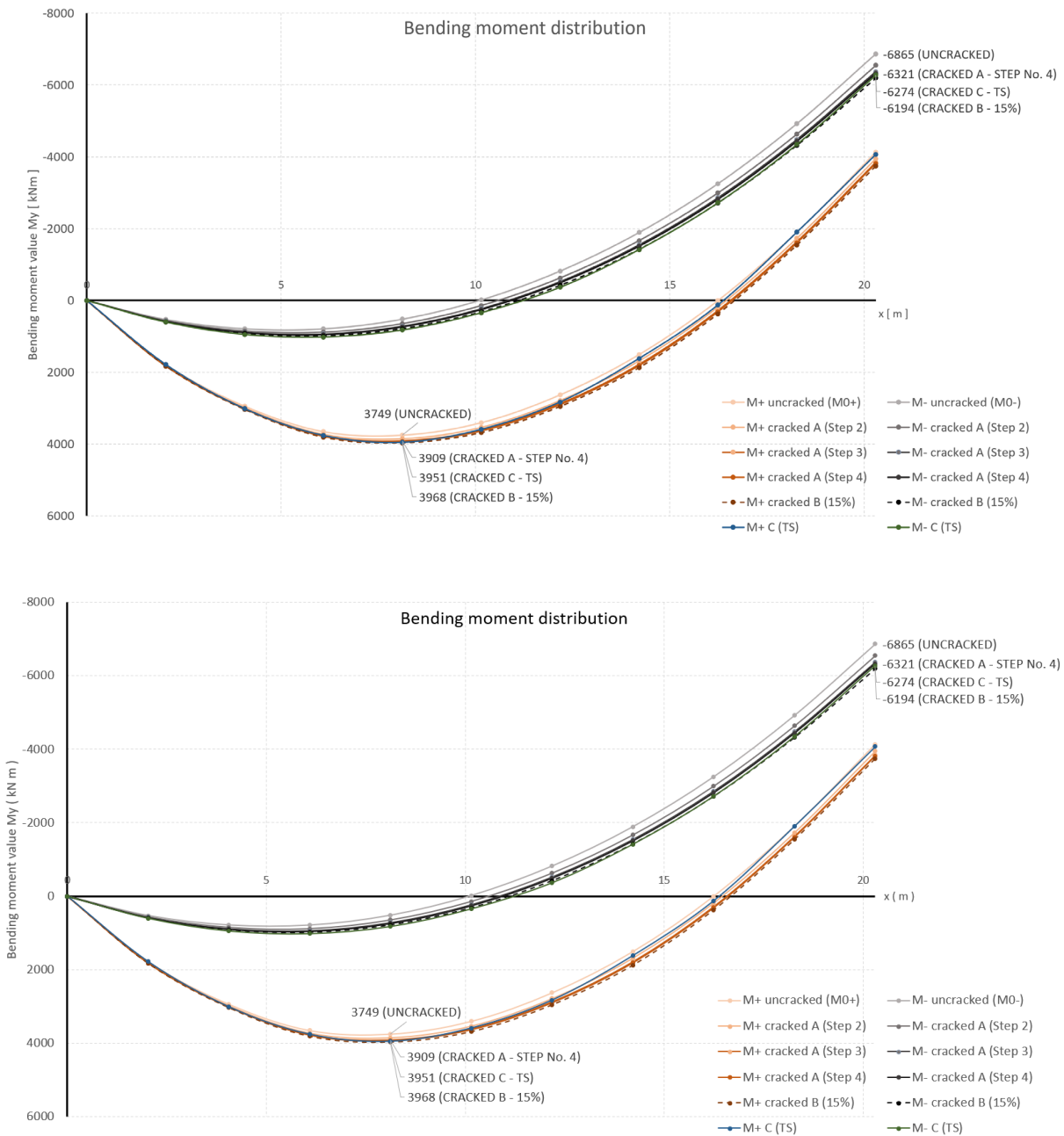
Figure 19: Bending moment envelope depending on the assumed approach (A, B, C).
