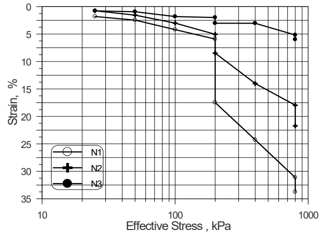
Figure 2: Results of collapse test for the three samples.
