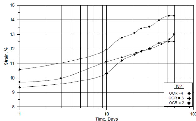
Figure 15: Variation of strain with time for the N2 soil. OCR: overconsolidation ratio.
