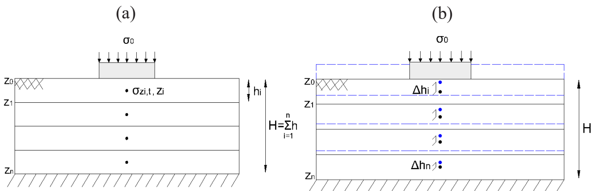
Figure 5: (a) Initial states of layers, (b) Final states of layers after total heave.
